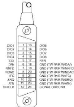
Figure 3.1 Rear Panel GPIB Connector
