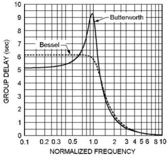
Figure 2.3 Group Delay
