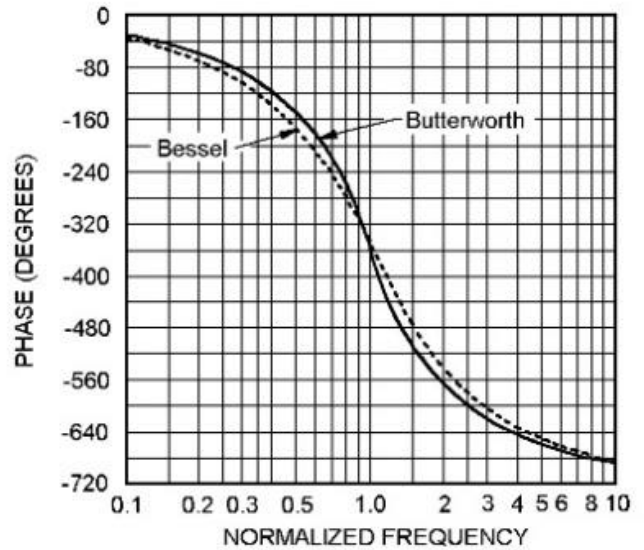
Figure 2.2 Phase Response
