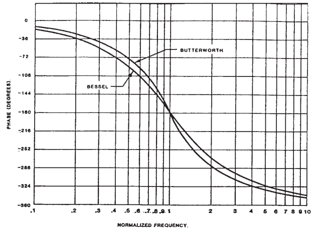
Phase Response
