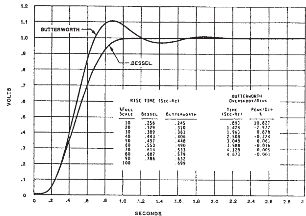
Transient Response
